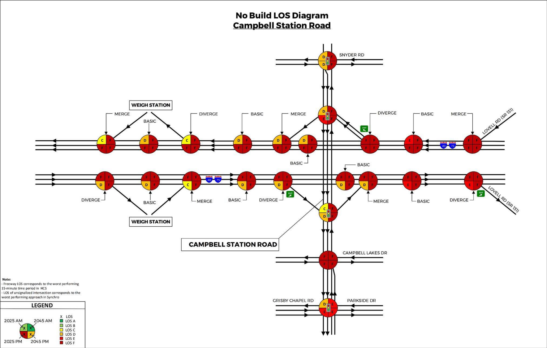
Figure 25. No-Build LOS Summary for Study Area (cont.)
